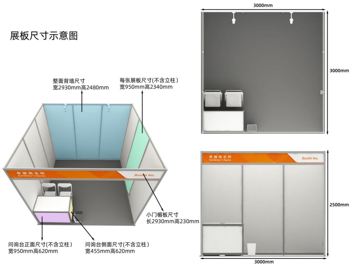
透视图 PRESPECTIVE VIEW
