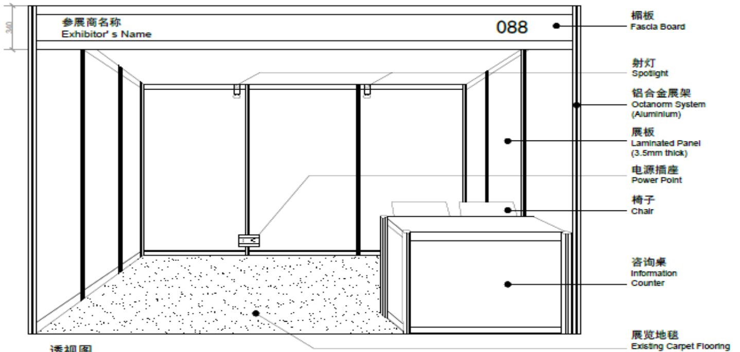
透视图 PERSPECTIVE VIEW
